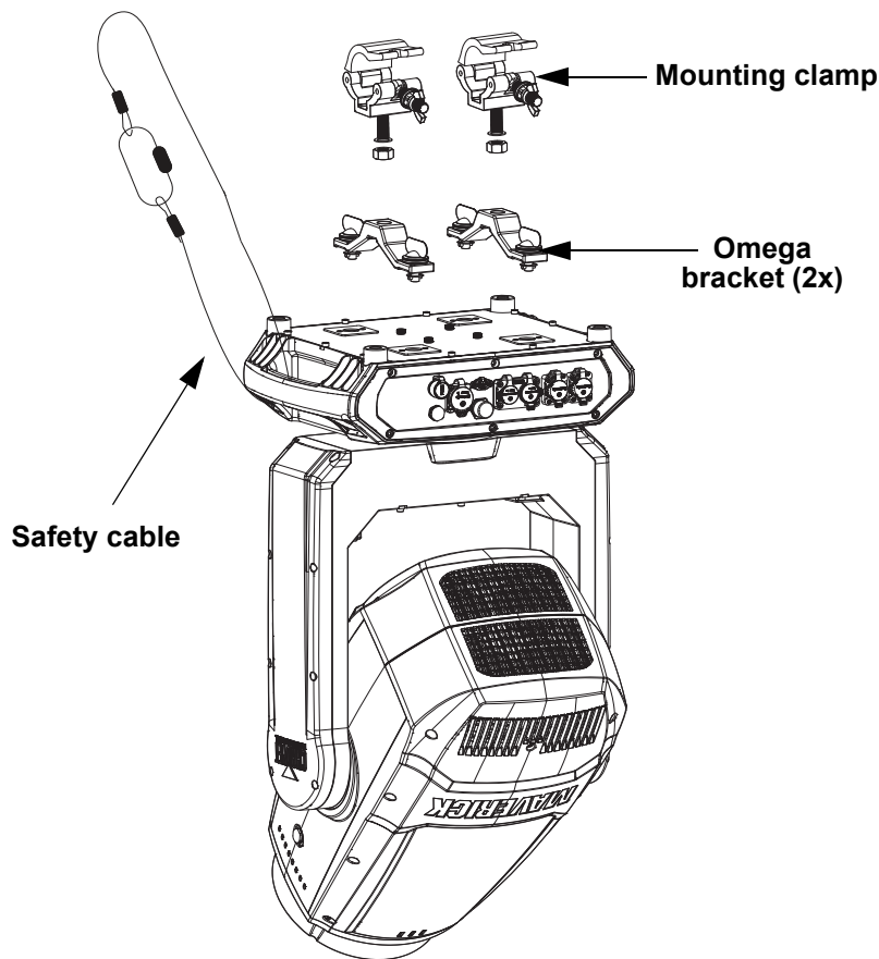
Overhead mounting
