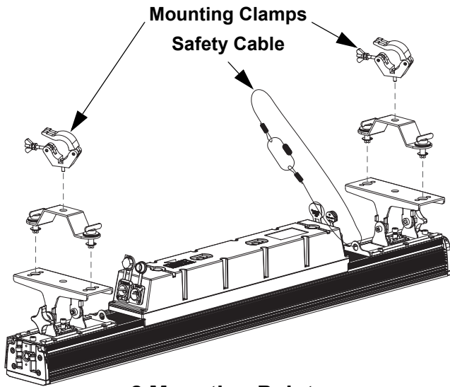
2 Mounting Points
