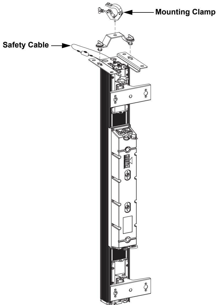
Overhead Mounting
